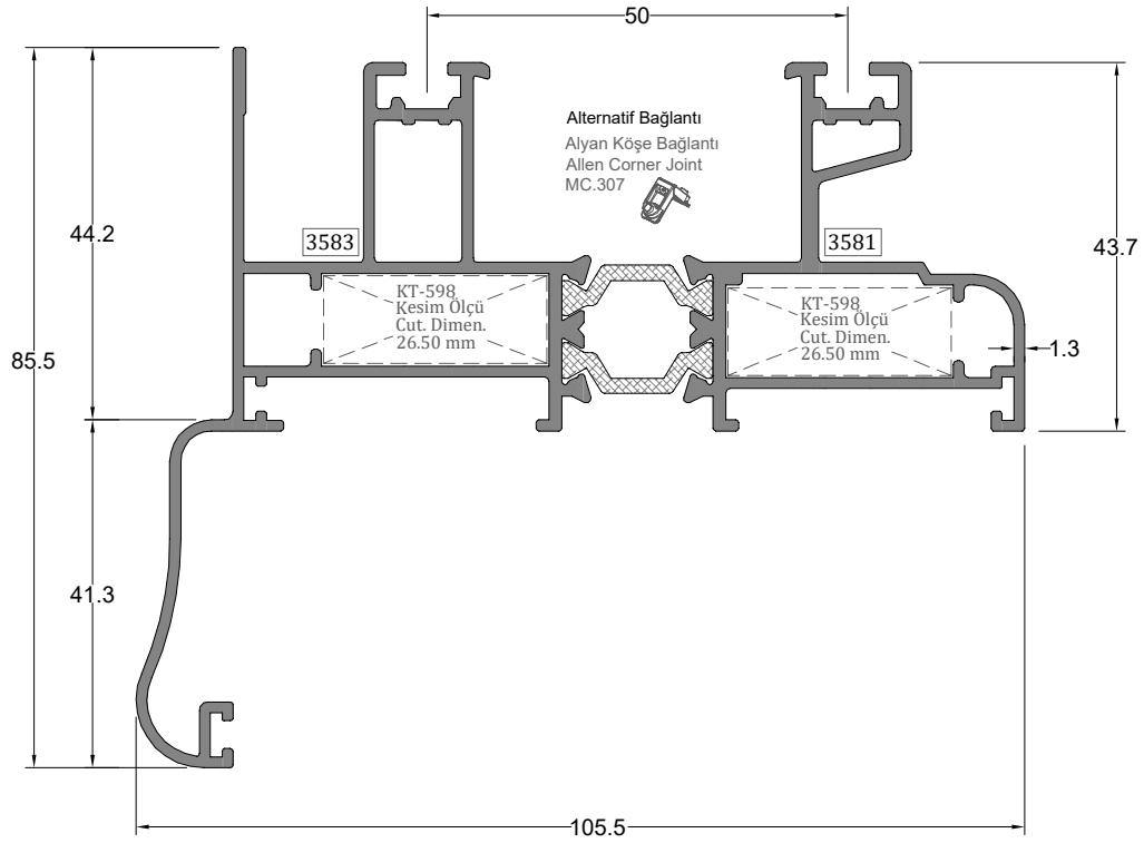
İki Raylı Kasa Profili DOUBLE RAIL FRAME PROFILE
