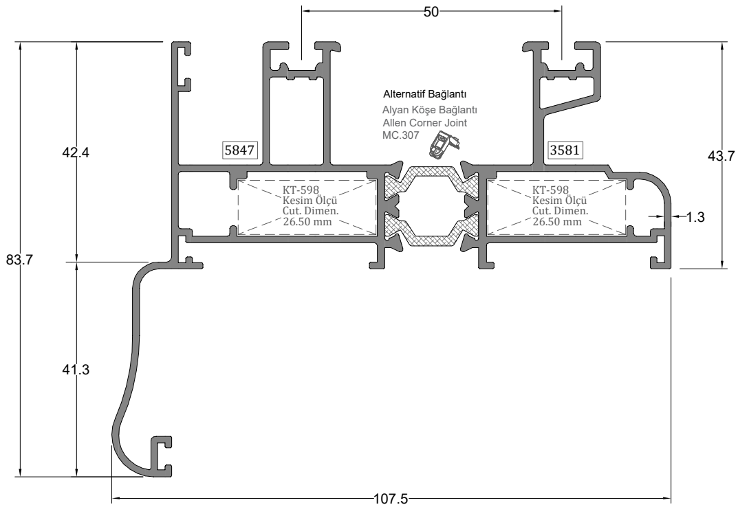
İki Raylı Kasa Profili DOUBLE RAIL FRAME PROFILE
